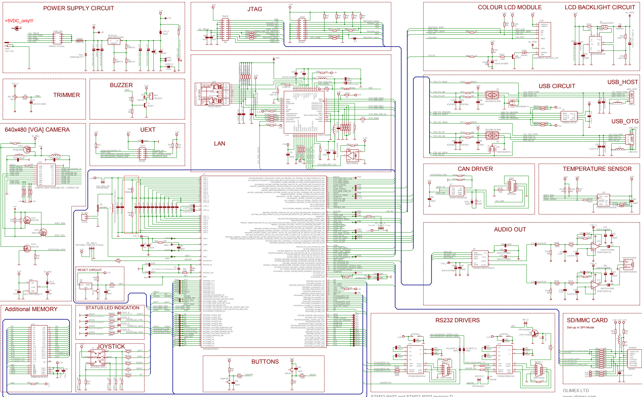
STM32-P407 and STM32-P207 revision D
