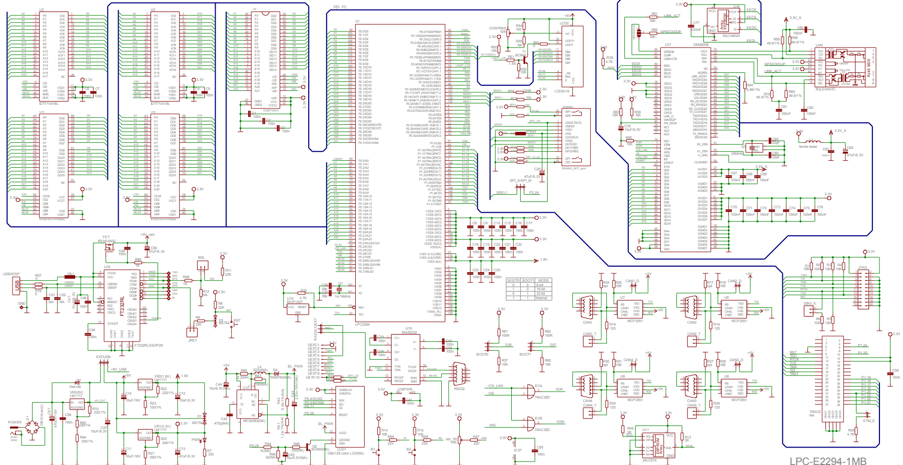
LPC-E2294-1MB Rev C COPYRIGHT(C) 2011, OLIMEX LTD. http://www.olimex.com/dev
