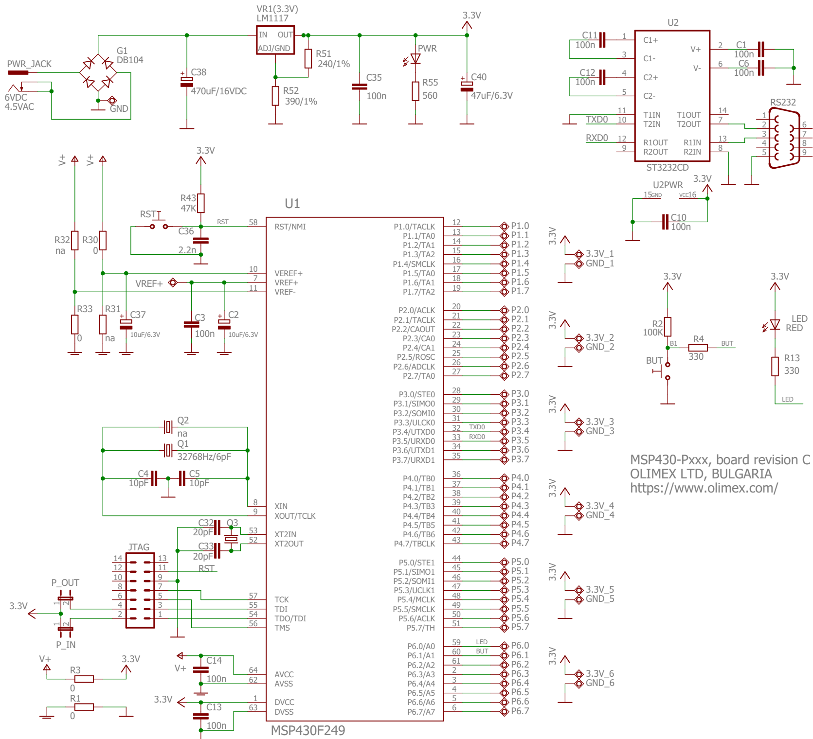
This schematic suits several Olimex boards. Among them are: MSP430-P149; MSP430-P169; MSP430-P249; MSP430-P1611; MSP430-P2618
